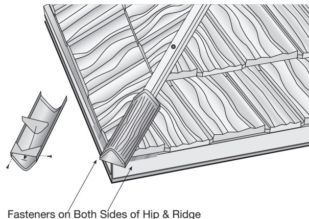
Fasteners on Both Sides of Hip & Ridge
